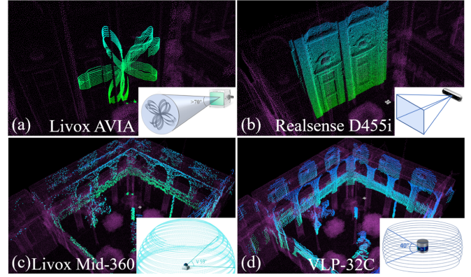
Fig. 10. Various LiDAR scan pattern support including Livox Avia (a), D455 (b), Livox Mid-360 (c), and VLP 32 (d), respectively.
